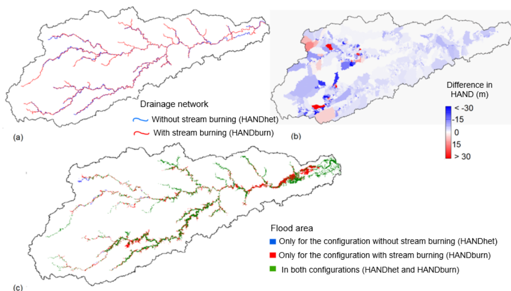
Figure 8 – (A) Comparison between river drainage networks obtained with and without stream burning; (B) Difference in HAND obtained using the DEM with and without stream burnings; (C) Analysis of flood areas obtained only for HAND without stream burning, only for HAND with stream burning, and simultaneously obtained with both.
