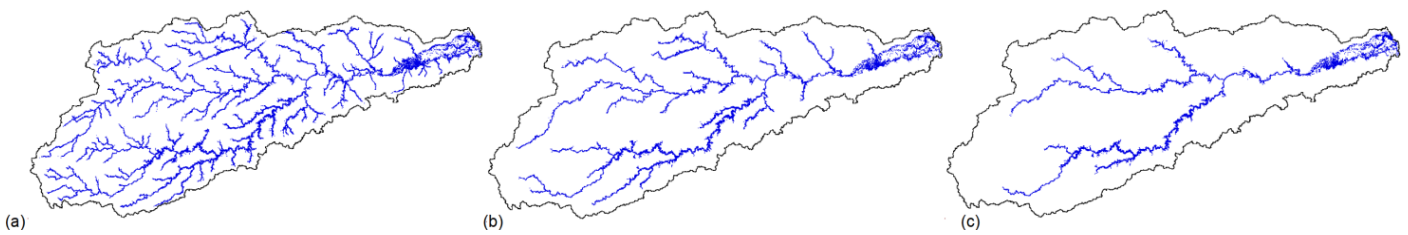
Figure 4 – Mapping of flood areas for a 5-m HAND threshold, considering a uniform minimum contributing area for drainage network initiation with values of (A) 5 km² (HANDu5); (B) 25 km² (HANDu10); and (C) 100 km² (HANDu100).
