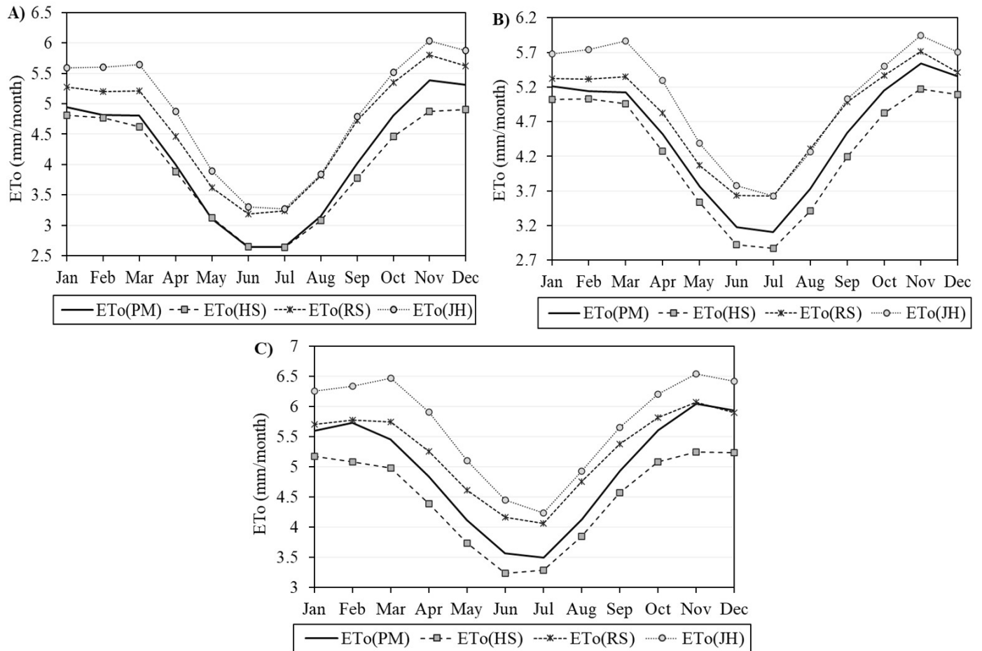
Figure 3 – ETo by ETo(PM), ETo(HS), ETo(RS), and ETo(JH) for the municipalities of A) Garanhuns, B) Caruaru, C) Surubim.
