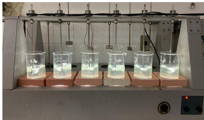
Figure 2 – Simulation of the coagulation, flocculation, and decantation stages in the Jar Test for the water from the Açude Grande.
