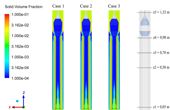
Figure 3 – Iso-surfaces of the sludge volume fraction distribution for cases 1, 2, and 3.
