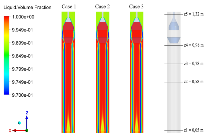
Figure 4 – Iso-surfaces of the water volume fraction distribution for cases 1, 2, and 3.
