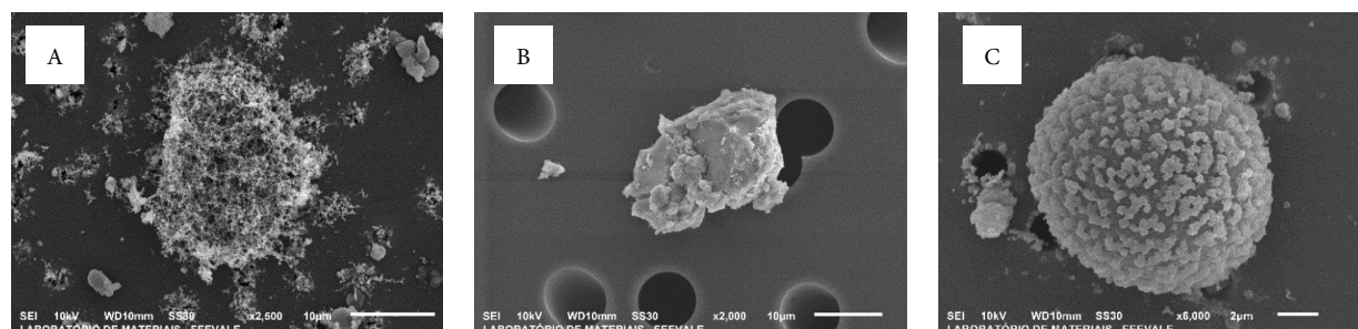
Figure 9 – Particles of varying origins identified in Gramado and Canela. Vehicle soot particle identified in PM 2.5 in Gramado (A); particles found in PM 2.5-10 in Canela (B); and particle found in PM 2.5 in Gramado (C).
