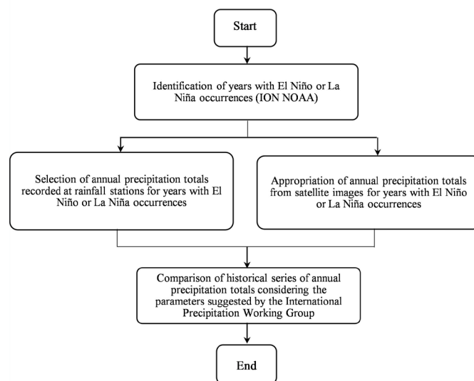
Figure 2 – Flowchart of activities for comparing annual total precipitation records obtained from rain gauges and estimated from satellite images, considering partial series for El Niño and La Niña years.
