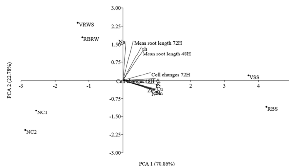
Figure 4 – Plot of the principal components analysis of the relationship between the chemical elements, watercourses, and cytogenotoxicity.
