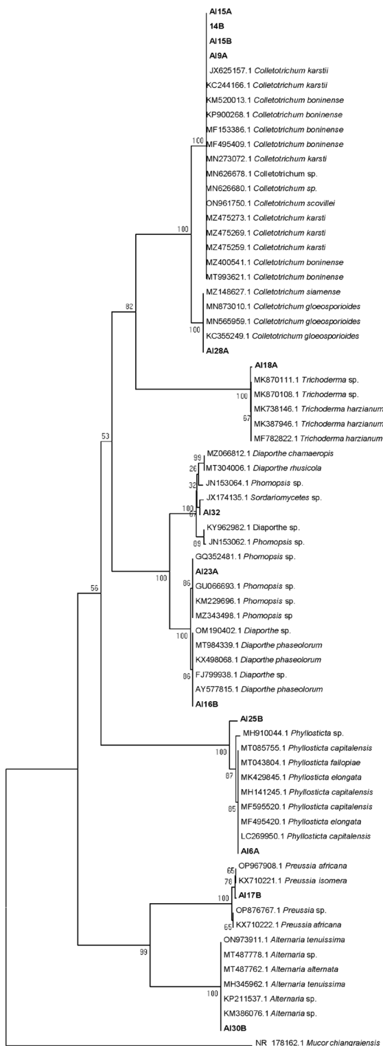
Figure 1 – Phylogenetic tree constructed with sequences of endophytic fungi isolated from Azadirachta indica and sequences from GenBank (indicated by the database code), through the neighbor-joining method using p-distance for nucleotides, with the option of pairwise gap deletion. The numbers above and below each node indicate the frequency (in percentage) of each branch in bootstrap analyses of 10,000 replicates.
