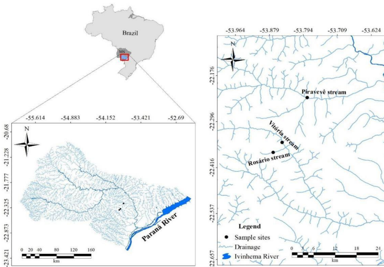
Figure 1 – Sampling sites located in Vitória, Rosário, and Piravevê streams, Ivinhema River basin, Mato Grosso do Sul, Brazil.
