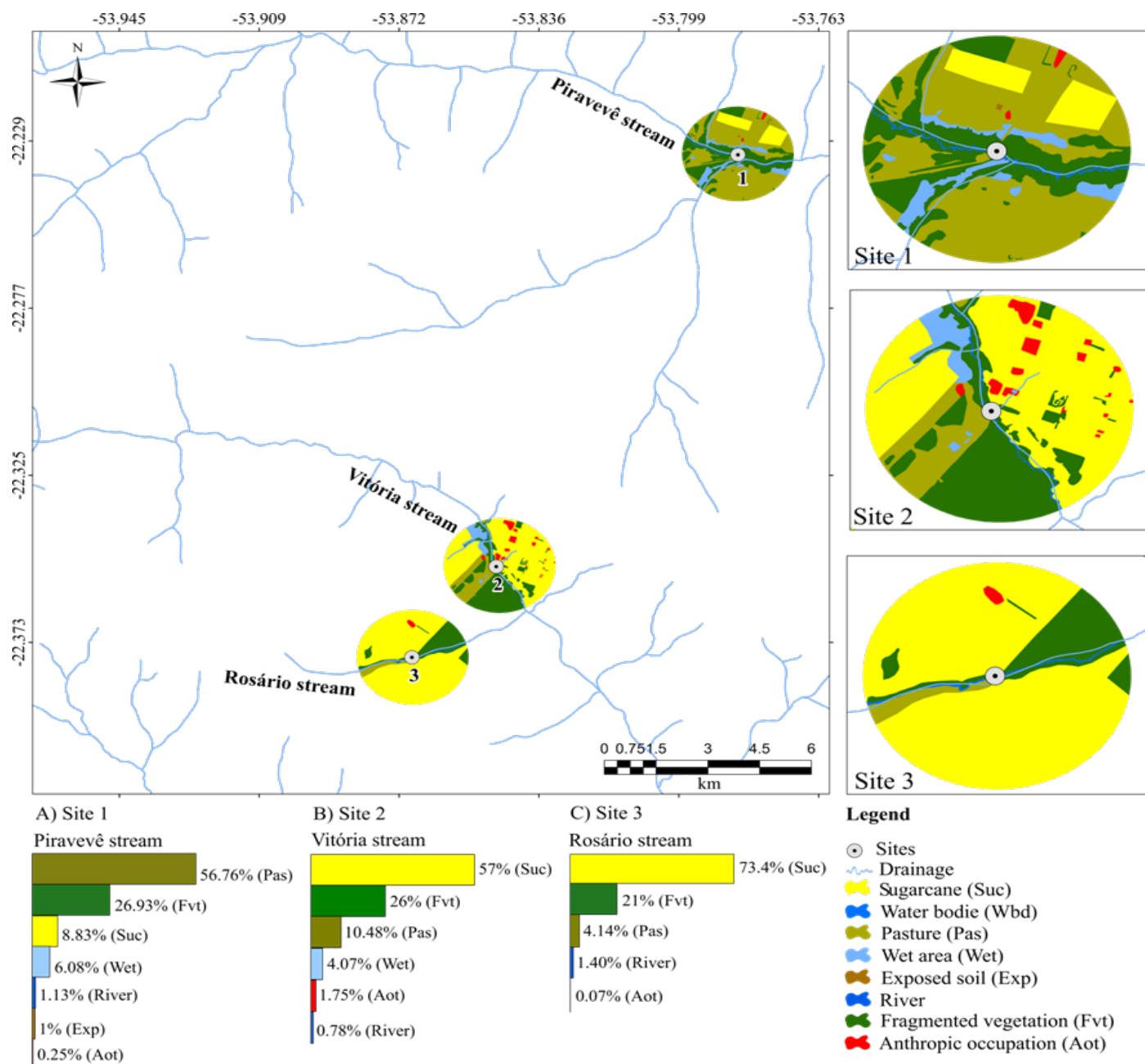
Figure 2 – Land use and cover around sampling sites located in Piravevê, Vitória, and Rosário streams, Ivinhema River basin, Mato Grosso do Sul, Brazil.
