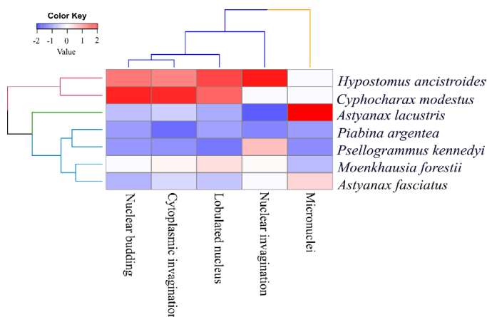
Figure 3 – Hierarchical clustering of the means of genotoxicity biomarkers observed in erythrocytes of fish species samples collected in situ in Piravevê, Vitória, and Rosário streams, Ivinhema River basin, in Mato Grosso do Sul, Brazil.
