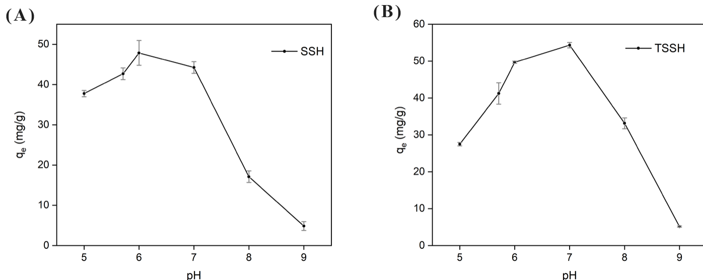
Figure 3 – Adsorption capacity at varying pHs for sunflower seed husks (A) and treated sunflower seed husks (B). SSH: sunflower seed husks; TSSH: treated sunflower seed husks; q_e : adsorption capacity at equilibrium; pH: potential of hydrogen.
