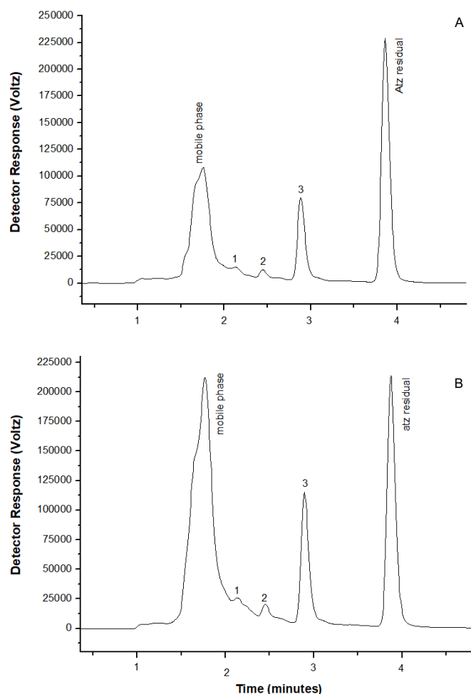
Figure 5 – Residual atrazine and metabolites verified at the end of the degradation tests (5 days) with (A) free and (B) immobilized P. chrysogenum NRRL 807. The numbered peaks refer to the degradation metabolites.
