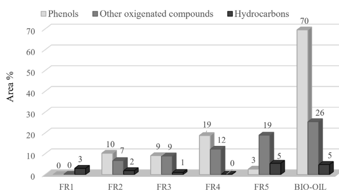
Figure 3 – Distribution of chemical classes: phenols, hydrocarbons, and other oxygenated compounds in the fractions and in the crude bio-oil analyzed by GC/qMS related to the yield of each fraction (yield corresponding to the chemical class x yield of the fraction). FR1: n-hexane; FR2: n-hexane/toluene; FR3: dichloromethane/toluene; FR4: acetone/dichloromethane; FR5: methanol.
