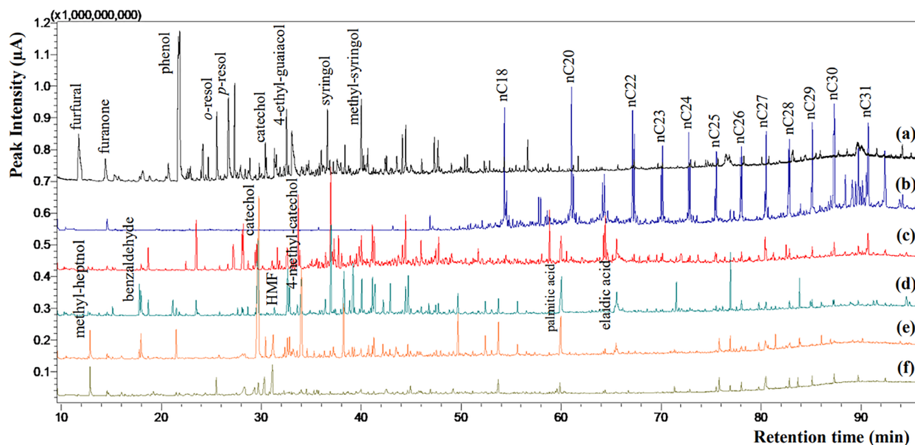
Figure 2 – Total ion chromatogram of the (A) bio-oil before fractionation; (B) FR1 — n-hexane; (C) FR2 — n-hexane/toluene; (D) FR3 — dichloromethane/toluene; (E) FR4 — acetone/dichloromethane; and (F) FR5 — methanol, in the SCAN mode. Chromatographic conditions are described in item 2.5 of the Methodological Procedures Section.
