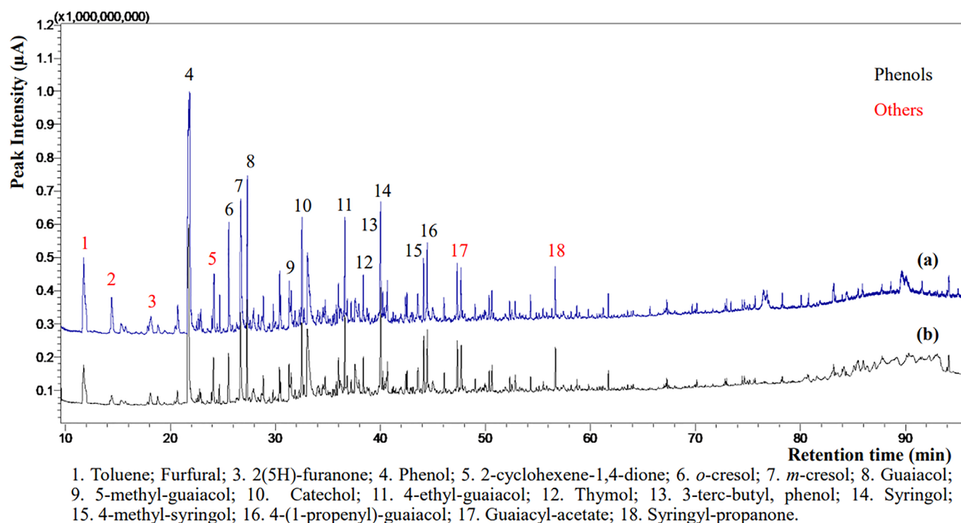
Figure 1 – Chromatographic profile of the bio-oils (GC/qMS SCAN mode) from coconut fibers: (A) BO100 and (B) BO200. Experimental conditions are described in item 2.5 of the Methodological Procedures Section. Majority compounds are identified in the chromatograms.
