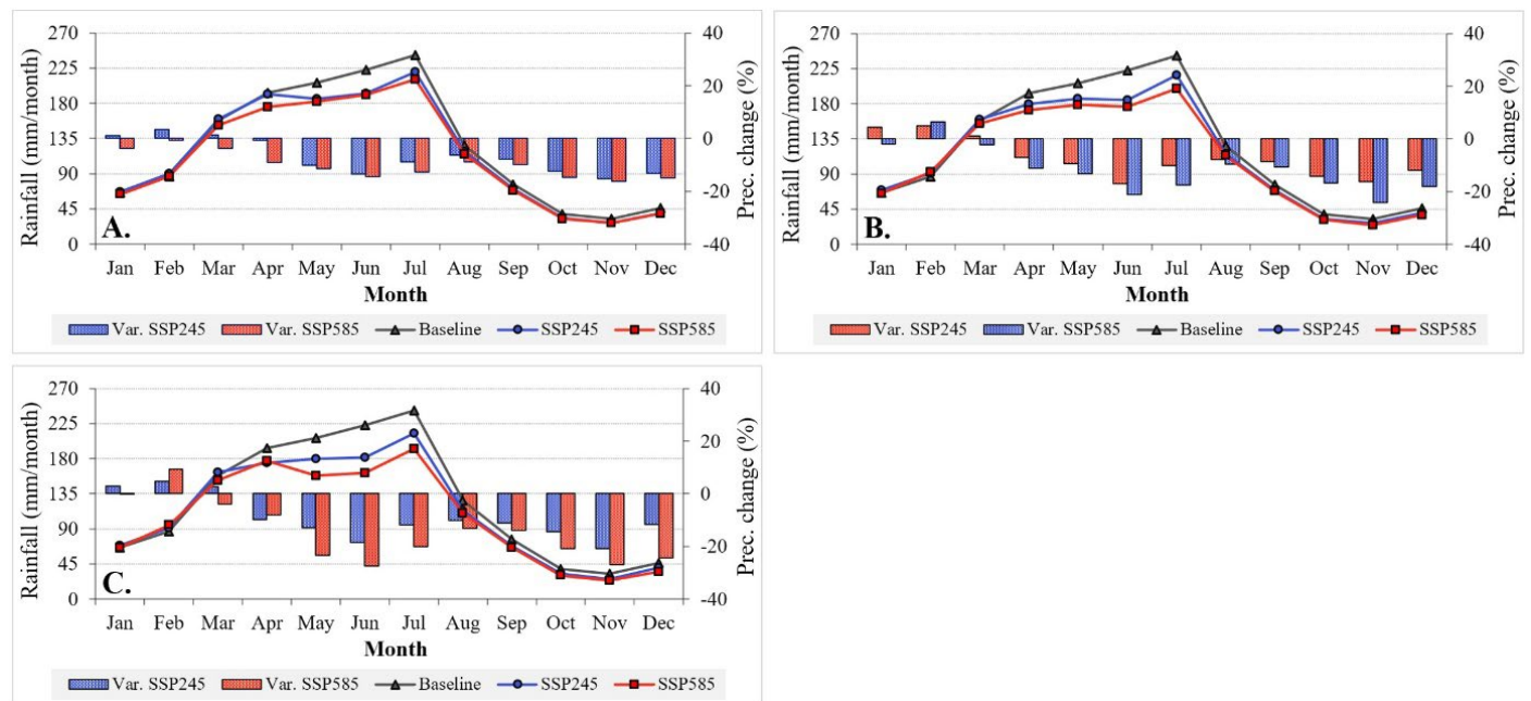
Figure 9 – Precipitation anomalies in the Zona da Mata of Pernambuco, based on Coupled Model Intercomparison Project Phase 6 models for the SSP245 and SSP585 scenarios, during the periods (A) 2041–2060, (B) 2061–2080, and (C) 2081–2100.
