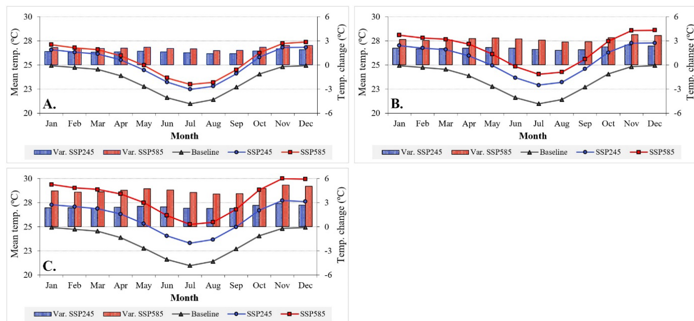
Figure 3 – Average temperature (baseline) and temperature change in Pernambuco, based on the Coupled Model Intercomparison Project Phase 6 models for the SSP245 and SSP585 scenarios, during the periods (A) 2041–2060, (B) 2061–2080, and (C) 2081–2100.
