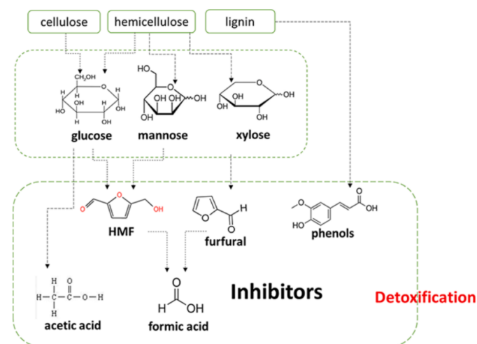
Figure 6 – Formation of furfural and hydroxymethylfurfural inhibitors. Source: Guo et al. (2022).
