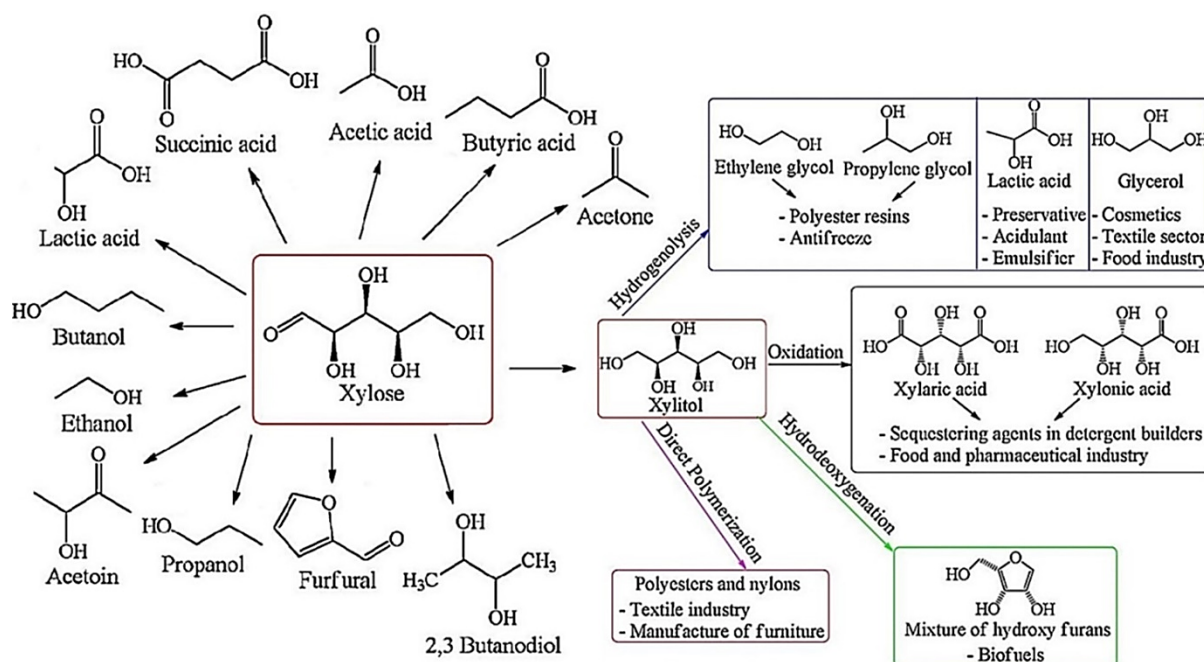
Figure 3 – Compounds obtained from xylose.
