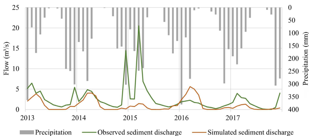
Figure 5 – Observed and simulated sediment discharges after calibration for the Capão Comprido Stream (DF, Brazil).
