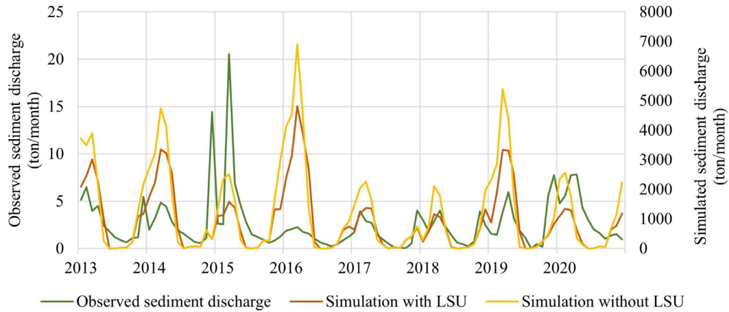
Figure 3 – Observed and simulated sediment discharge without calibration in the Capão Comprido Stream Basin (DF, Brazil).
