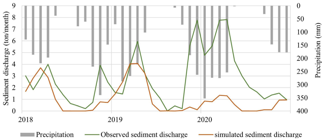
Figure 7 – Observed and simulated solid discharge for verification in the Capão Comprido Stream Basin (DE, Brazil).
