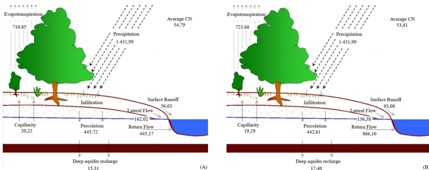
Figure 8 – (A) Simulated hydrological cycle in the Capão Comprido Stream Basin (DF, Brazil), without discretization in landscape units, with the Soil and Water Assessment Tool model, from 2006 to 2015. (B) Simulated hydrological cycle in the Capão Comprido Stream Basin (DF, Brazil), with discretization into landscape units, with the Soil and Water Assessment Tool model, from 2006 to 2015.
