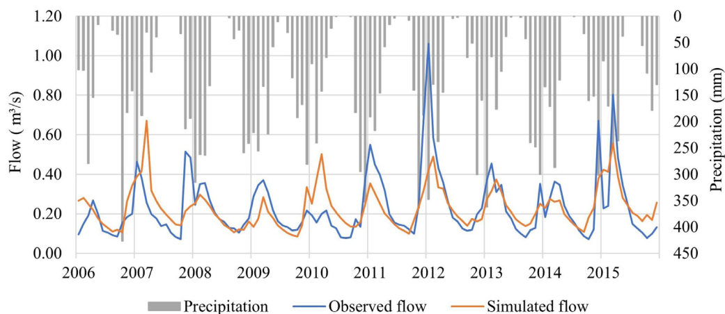
Figure 4 – Observed and simulated flows after the calibration process for the Capão Comprido Stream (DF, Brazil).
