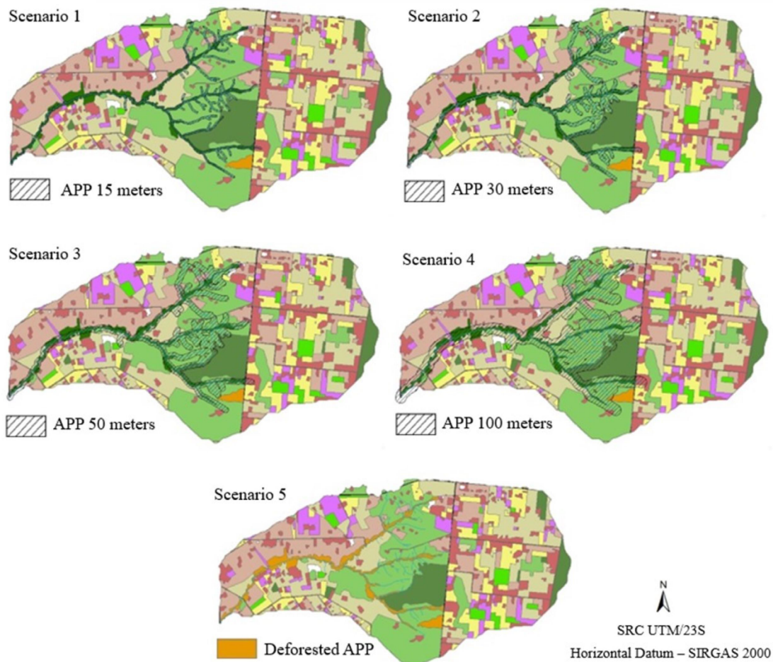
Figure 9 – Scenarios with permanent preservation areas of 15, 30, 50, and 100 m in length and a scenario with conversion of preserved permanent preservation areas to exposed soil in the Capão Comprido Stream watershed (DF, Brazil).
