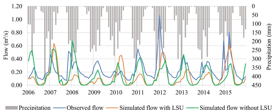
Figure 2 – Observed and simulated flows without calibration in the Capão Comprido Stream Basin (DF, Brazil).
