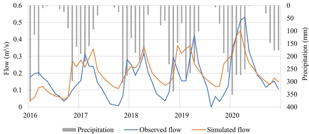
Figure 6 – Observed and simulated flow for verification in the Capão Comprido Stream Basin (DE, Brazil).
