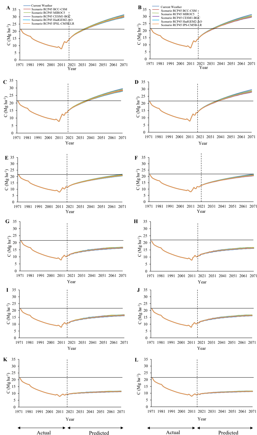
Figure 1 – Actual and predicted carbon stock by the RothC 2.3 model in five climate models in 6 multifunctional designs in an argisol cultivated with melon in the Brazilian semi-arid region modeled in the period 1971–2071.
