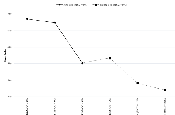
Figure 4 – Burst index.
