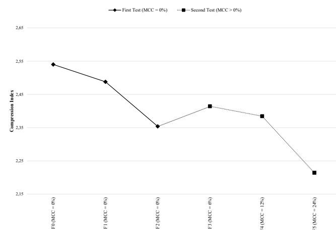
Figure 3 – Compression index.
