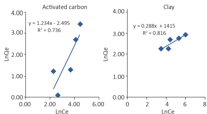
Figure 11 – Freundlich isotherm.
