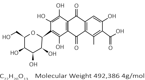
Figure 1 – Chemical structure of carmine.
