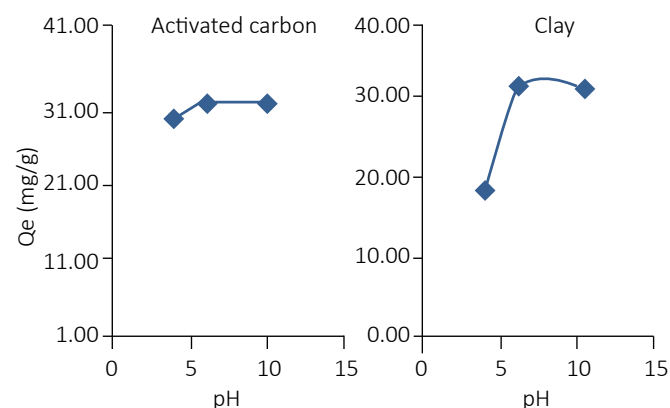
Figure 8 – The effect of changing the pH.
