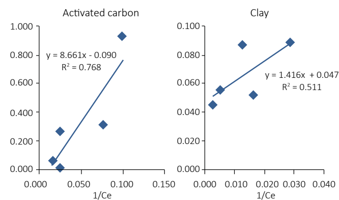
Figure 12 – Langmuir isotherm.
