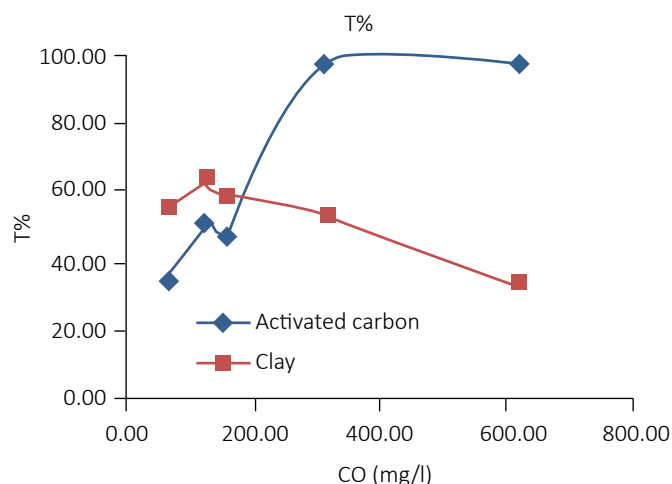
Figure 10 – Decolorization.
