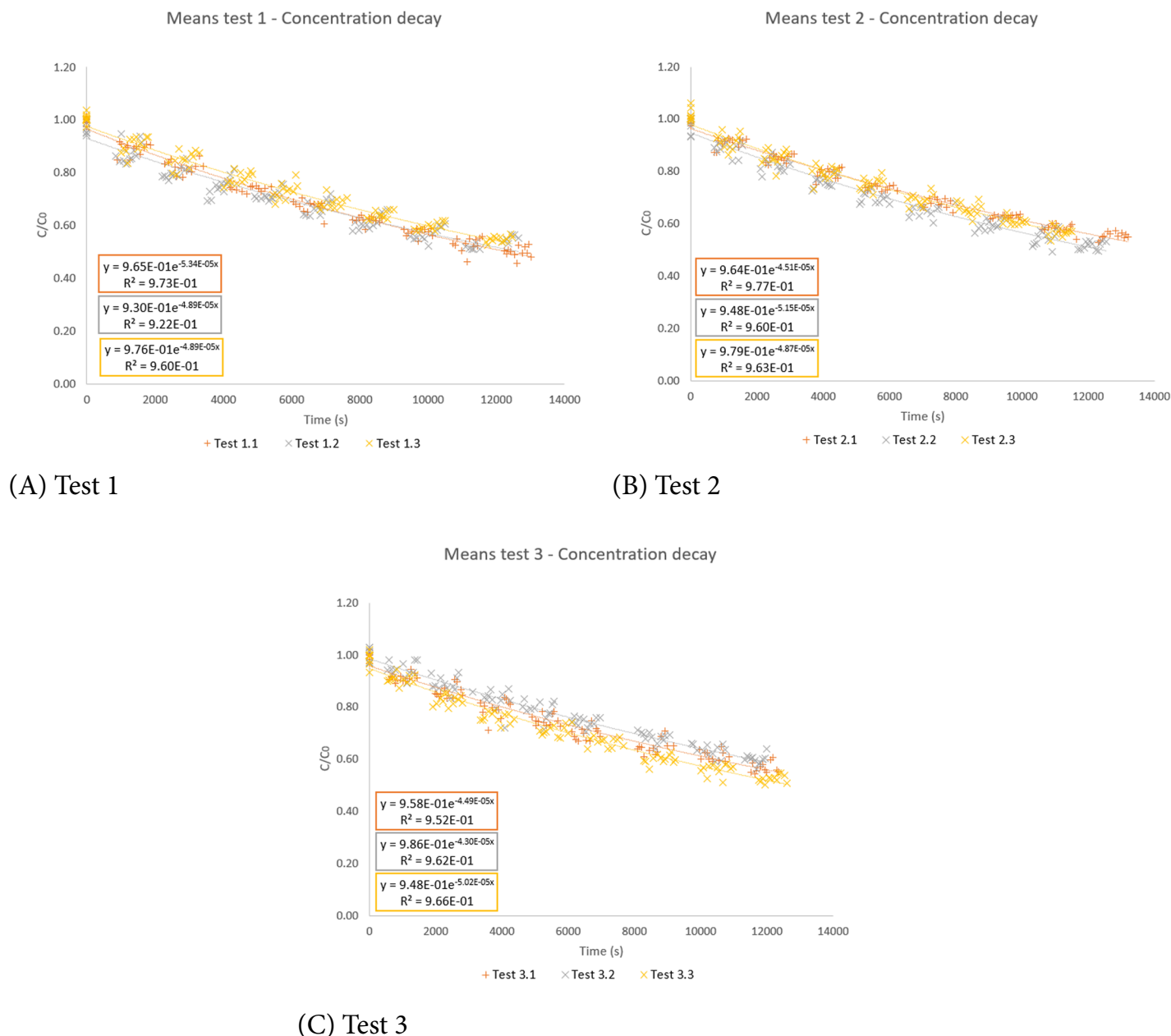
Figure 2 – Exponential adjustment for the mean of all points to obtain the global mass transfer coefficient.
