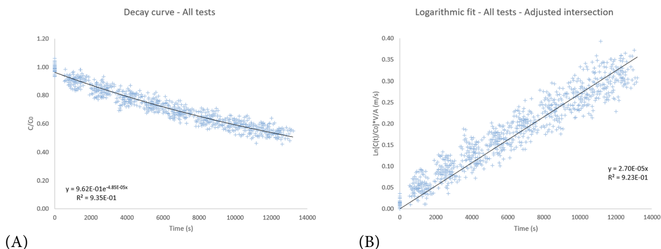
Figure 6 – Adjustments considering all the tests to evaluate (A) concentration decay with exponential adjustment and (B) the obtention of the global mass transfer coefficient with linear adjustment and forced intersection at the origin, applied to the equation in logarithmic form.
