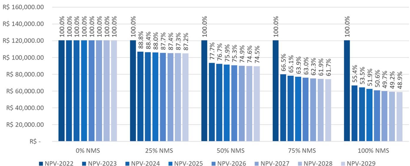
Figure 5 – Net present value as a function of the installation year and percentage use of the energy compensation system for system #3.
