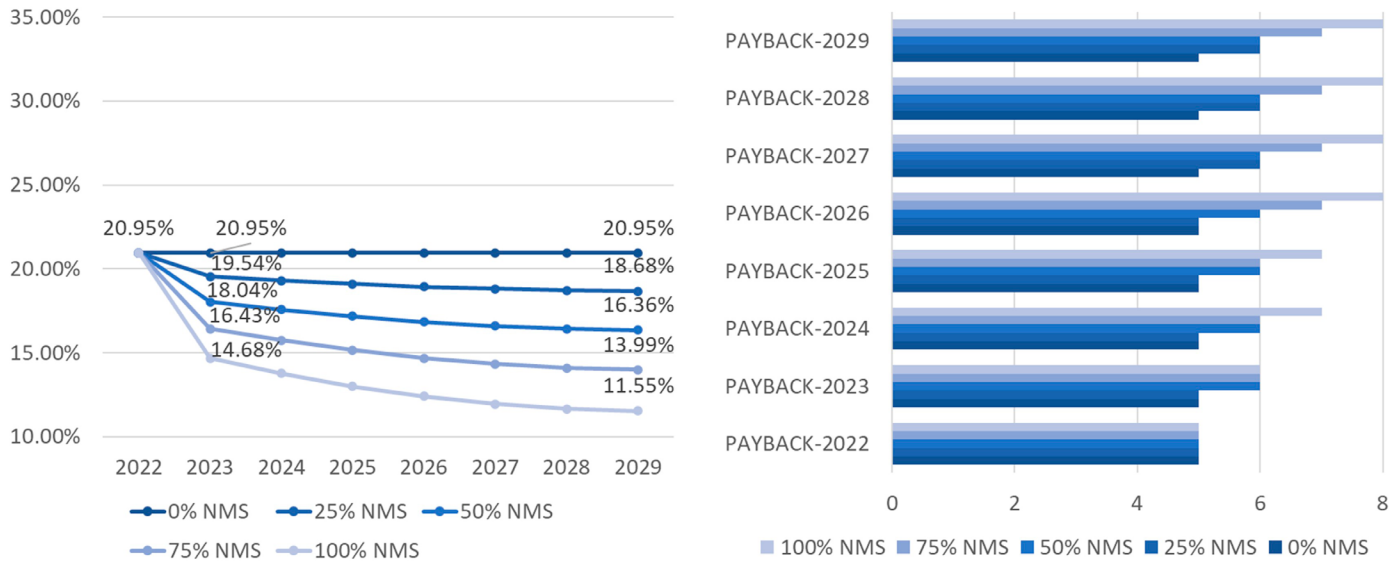
Figure 6 – Variation of the (A) internal rate of return and (B) payback for system #3.
