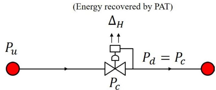
Figure 3 – Energy dissipated by PRV and recovered by PAT.
