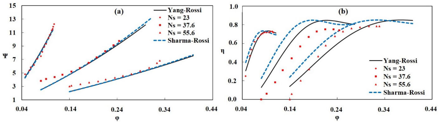
Figure 5 – Curves (A) \psi - \phi and (B) \eta - \phi .
