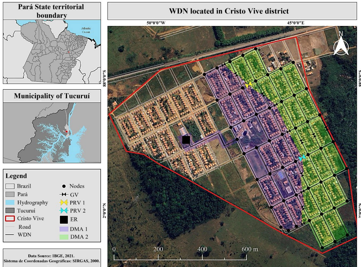
Figure 4 – WDN divided into two DMAs using two PRVs.
