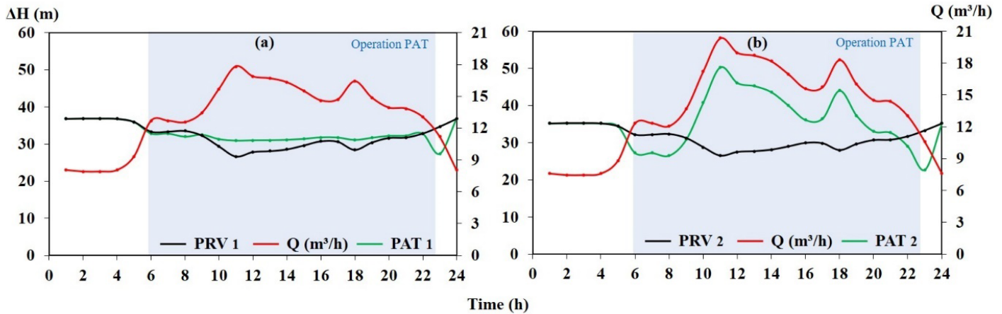
Figure 6 – PAT 1 \Delta H comparison and (A) PRV 1 PAT 2 and (B) PRV 2 at constant speed.
