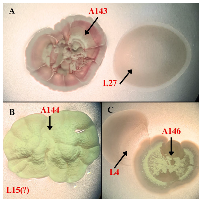
Figure 1 – Examples of co-inoculation test results. (A) Interaction between L27 rhizobia and A143 Actinobacteria strains in the medium with xylan. (B) Absence of interaction between the L15 rhizobia (inoculated on the left side of the image, where there was no growth) and A144 Actinobacteria strains in the medium with xylan. (C) Antagonistic interaction between L4 rhizobia and A146 Actinobacteria strains in the medium with CMC. The Actinobacteria produced a halo of rhizobia growth inhibition.
