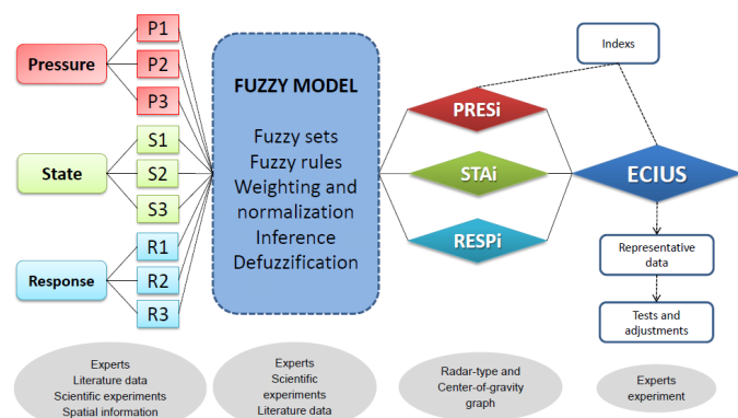
Figure 3 – Structure of the system based on fuzzy rules for calculating the Environmental Conservation Index of Urban Streams (ECIUS).
