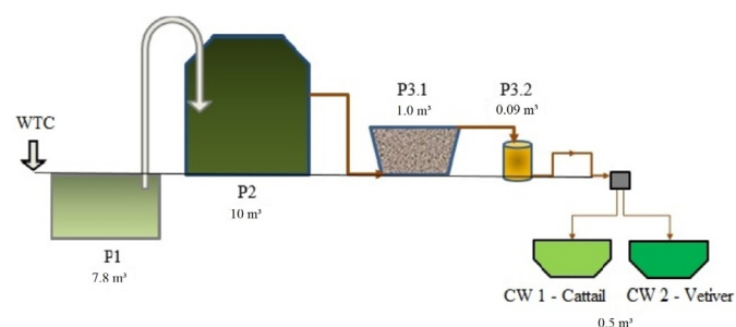
Figure 1 – Flowchart of the stages of the PTU: P1 – dung; P2 – septic tank; P3.1 – upward flow filter; P3.2 – downward flow filter; and CWs – beds grown with cattail ( Typha domingensis ) and Vetiver grass ( Chrysopogon zizanioides ). WTC: wastewater from treated cattle.
