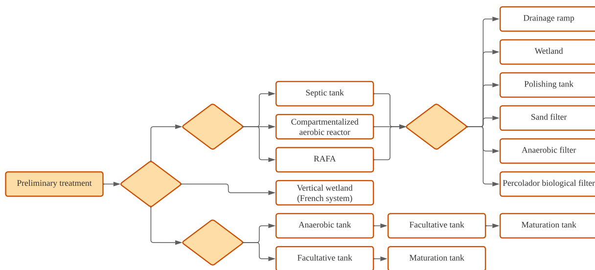
Figure 1 – Technological matrix of sewage collection and treatment solutions, according to PNSR.
