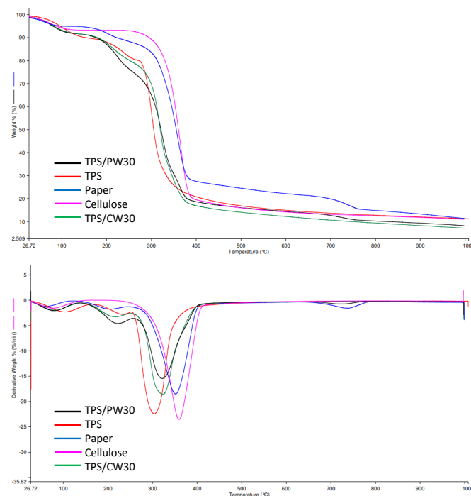
Figure 4 – TPS/PW30, TPS, Paper, Cellulose, and TPS/CW30 (A) TG and (B) DTG (no weathering).
