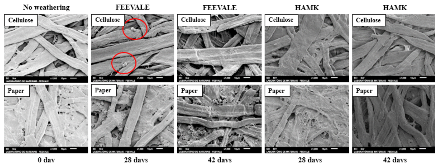
Figure 7 – Micrographs (1000x) of cellulose and paper before and after the weathering period at Universidade Feevale and HAMK.
