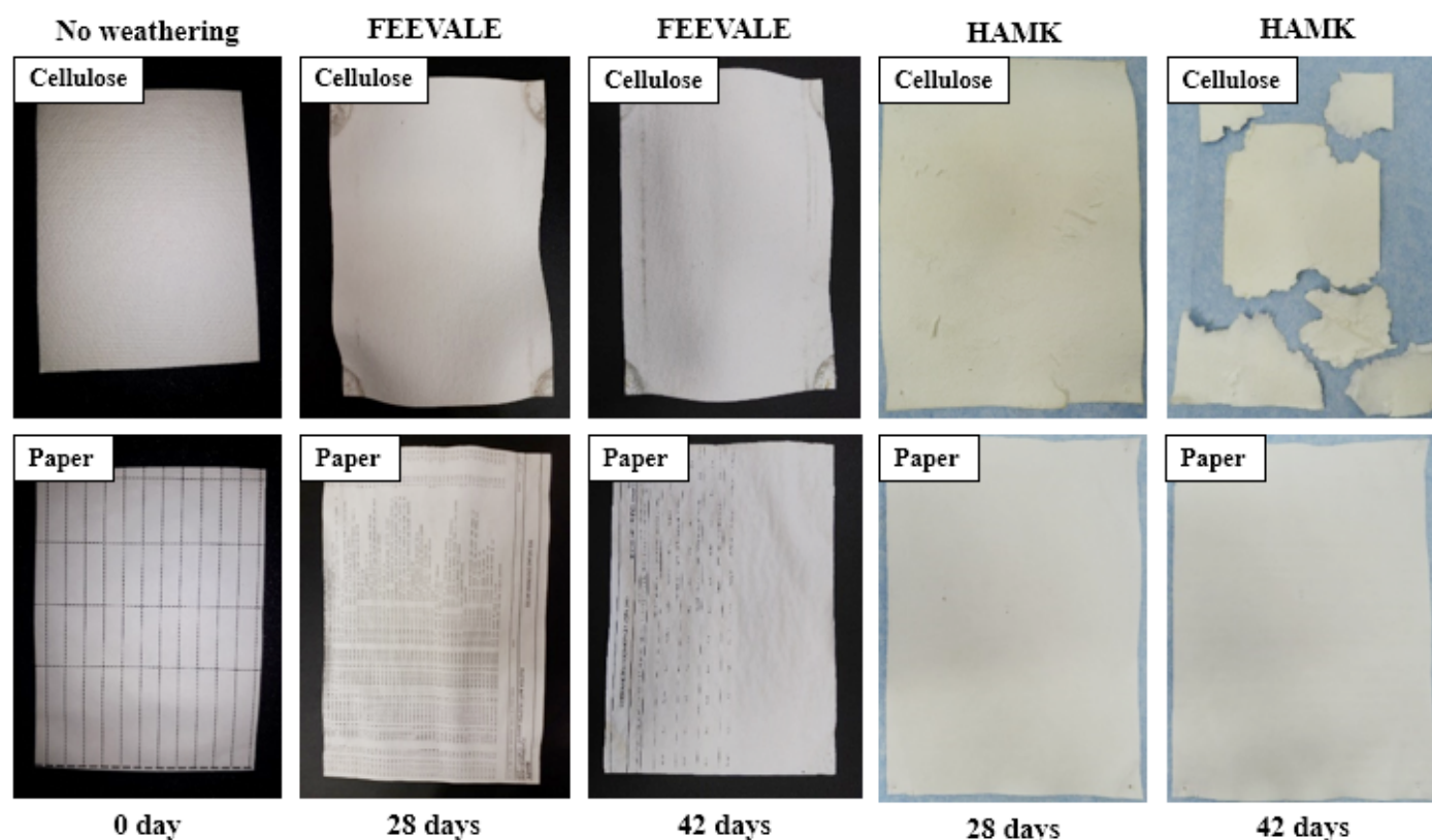
Figure 10 – Photographs of cellulose and paper before and after the weathering period at Universidade Feevale and HAMK.
