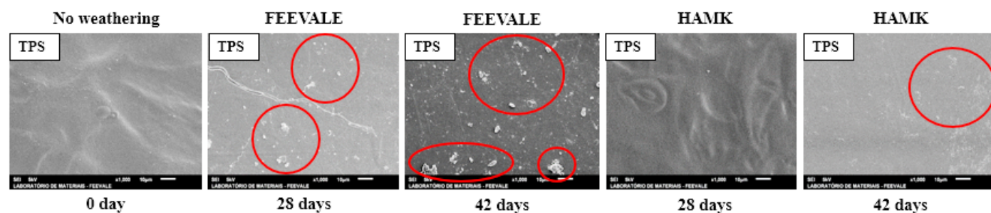
Figure 6 – Micrographs (1000x) of TPS before and after the weathering period at Universidade Feevale and HAMK.
