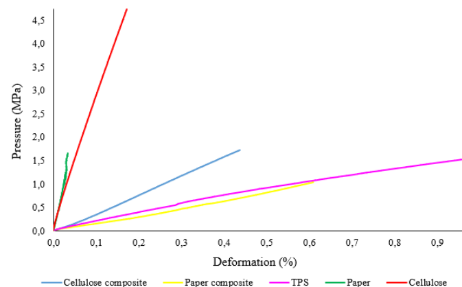
Figure 5 – Stress x deformation curves of TPS/CW30, TPS/PW30, TPS, paper, and cellulose (no weathering).
