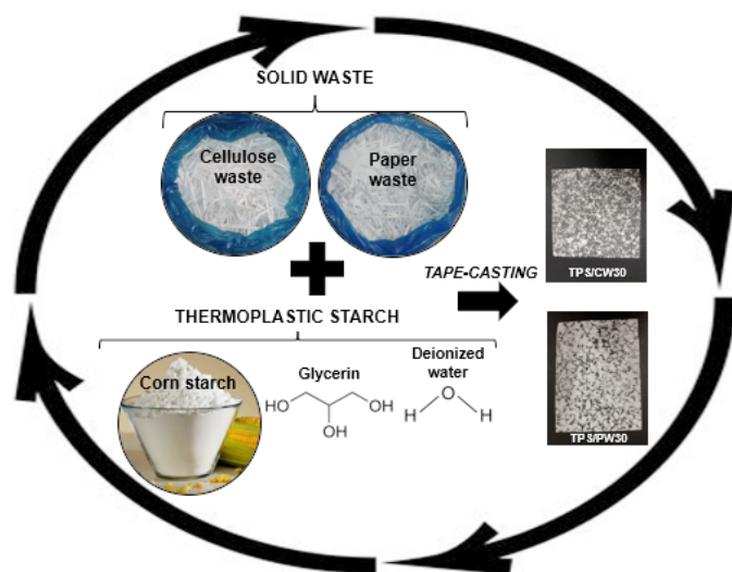
Figure 1 – Obtaining samples of TPS/CW30 and TPS/PW30.
