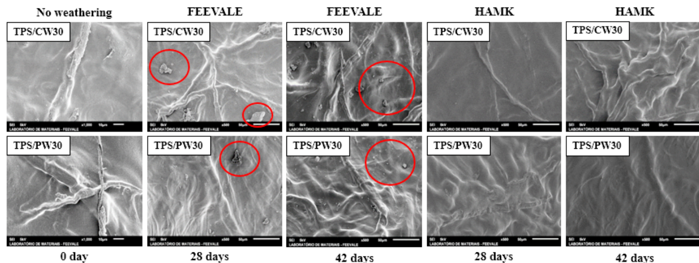
Figure 8 – Micrographs (500x and 1,000x) of TPS/CW30 and TPS/PW30 before and after the weathering period at Universidade Feevale and HAMK.
