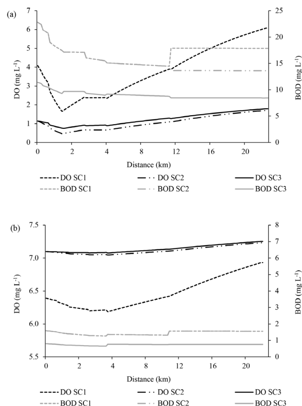
Figure 4 – Simulated values of dissolved oxygen (DO) and biochemical oxygen demand (BOD) for the three different scenarios (SC) in the (A) dry and (B) rainy seasons.
