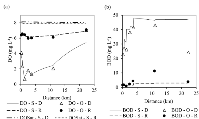
Figure 3 – Values of dissolved oxygen (DO), oxygen saturation concentration (DOSat) and biochemical oxygen demand (BOD) observed (O) in the Paraíba River and simulated (S) by QUAL2K during the first and second sampling campaigns in the dry (D) (09/05/2019) and rainy (R) (03/03/2020) seasons.
