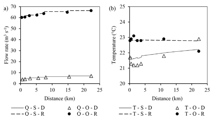
Figure 2 – Flow rate (Q) and temperature (T) values observed (O) in the Paraibuna River and simulated (S) by QUAL2K during the first and second sampling campaigns in dry (D) (May 09, 2019) and rainy (R) (March 03, 2020) seasons.
