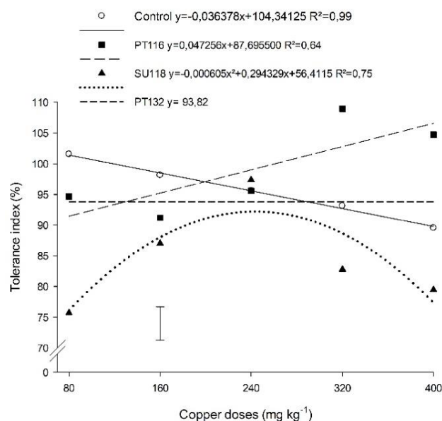
Figure 4 – Relationship between the Tolerance Index (ITOL) of Ilex paraguariensis seedlings with the doses of copper applied in the soil, control treatments without inoculation (Control) and with the addition of three inocula of ectomycorrhizal fungi Pisolithus microcarpus (PT116), Pisolithus tinctorius (PT132), and Suillus cothurnatus (SU118). DMS: minimum significant difference by Tukey's test ( p \leq 0.05 ).
