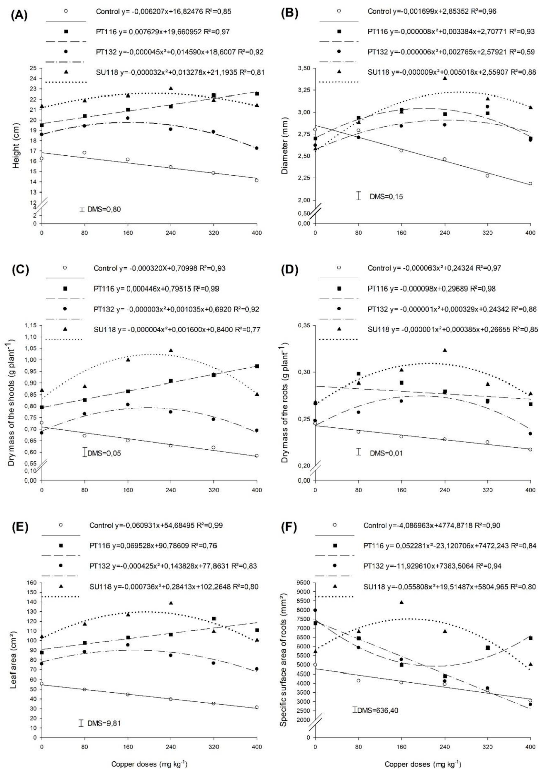
Figure 2 – (A) Ratio of height, (B) stem diameter — Diameter, (C) dry mass of the shoots — MSPA, (D) dry mass of the roots — MSR, (E) leaf area, and (F) specific surface area of the roots — ASE of Ilex paraguariensis seedlings with copper doses applied in the soil, without (control — test) and with the addition of three inocula of ectomycorrhizal fungi such as Pisolithus microcarpus (PT116), Pisolithus tinctorius (PT132), and Suillus cothurnatus (SU118). DMS: minimum significant difference by Tukey's test ( p \leq 0.05 ).
