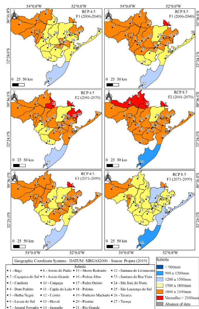
Figure 5 – Average total annual rainfall for cities of the Southern and Steppe regions, according to the CANESM2-ETA model, scenario RCP 4.5 and RCP 8.5, for the three future periods (F1, F2 and F3). Source: elaborated by the authors.
