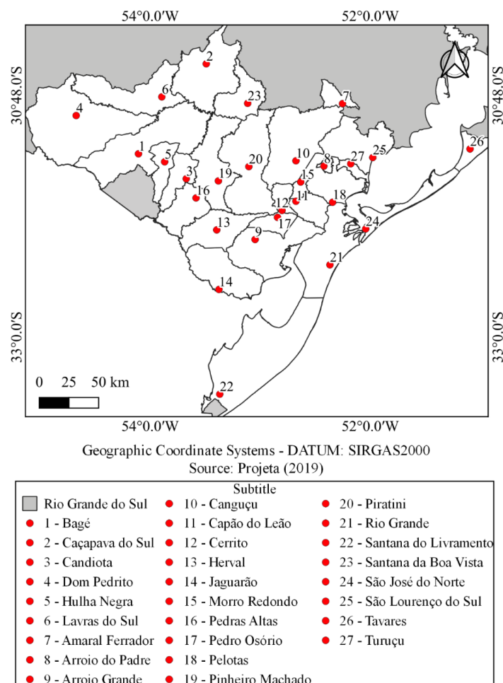
Figure 2 – Points of the climate models in each city in the study area.
