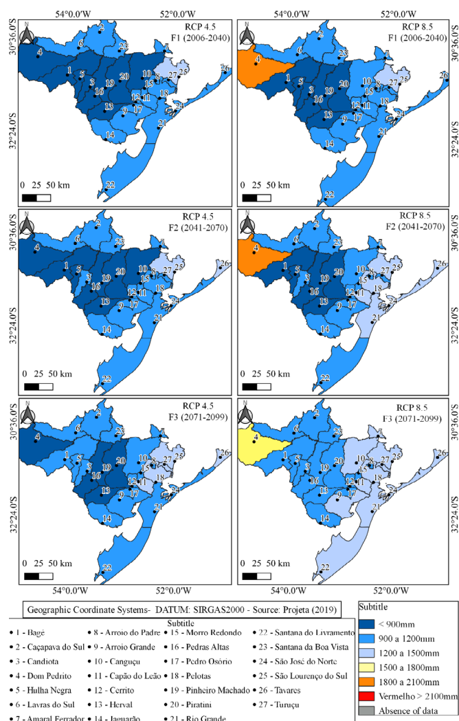
Figure 7 – Average total annual rainfall for cities of the Southern and Steppe regions, according to the MIROC5-ETA model, scenario RCP 4.5 and RCP 8.5, for the three future periods (F1, F2 and F3).
