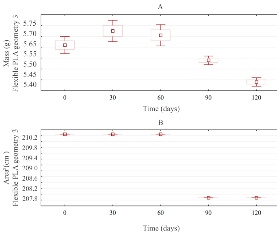
Figure 14 – Analysis of the (A) loss of mass (g) and (B) area (cm 2 ) by degradation of 3D-printed flexible PLA biopolymer (geometry 3) buried for 0, 30, 60, 90, and 120 days.
