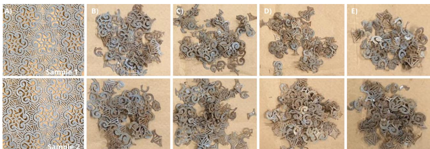
Figure 17 – Degradation process of 3D-printed rigid PLA biopolymer samples (geometry 3) buried for (A) 0, (B) 30, (C) 60, (D) 90, and (E) 120 days.
