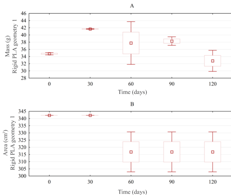
Figure 8 – Analysis of the (A) loss of mass (g) and (B) area (cm 2 ) by degradation of 3D-printed rigid PLA biopolymer (geometry 1) buried for 0, 30, 60, 90, and 120 days.
