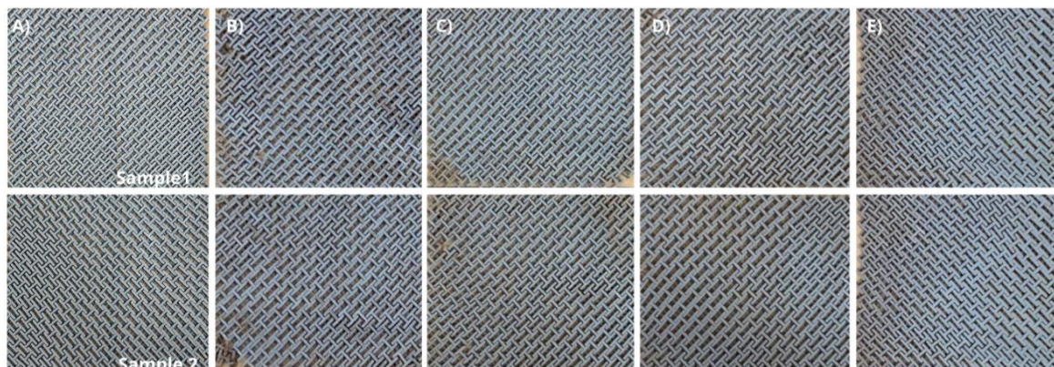
Figure 13 – Degradation process of 3D-printed rigid PLA biopolymer samples (geometry 2) buried for (A) 0, (B) 30, (C) 60, (D) 90, and (E) 120 days.
