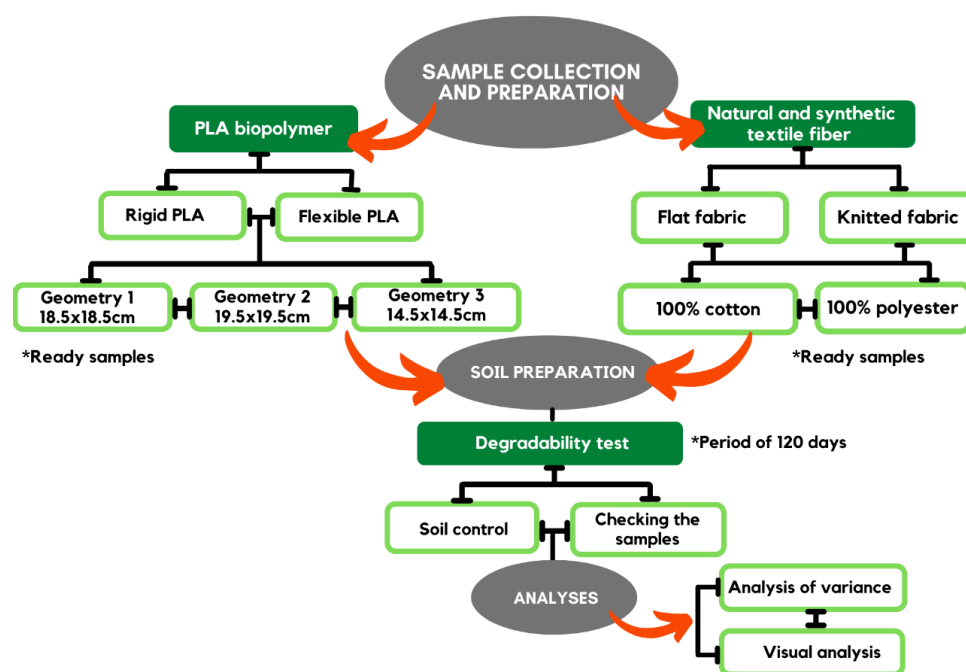
Figure 1 – Flowchart of the methodology used for degradation of flexible and rigid PLA biopolymer samples, natural and synthetic fiber fabrics.
