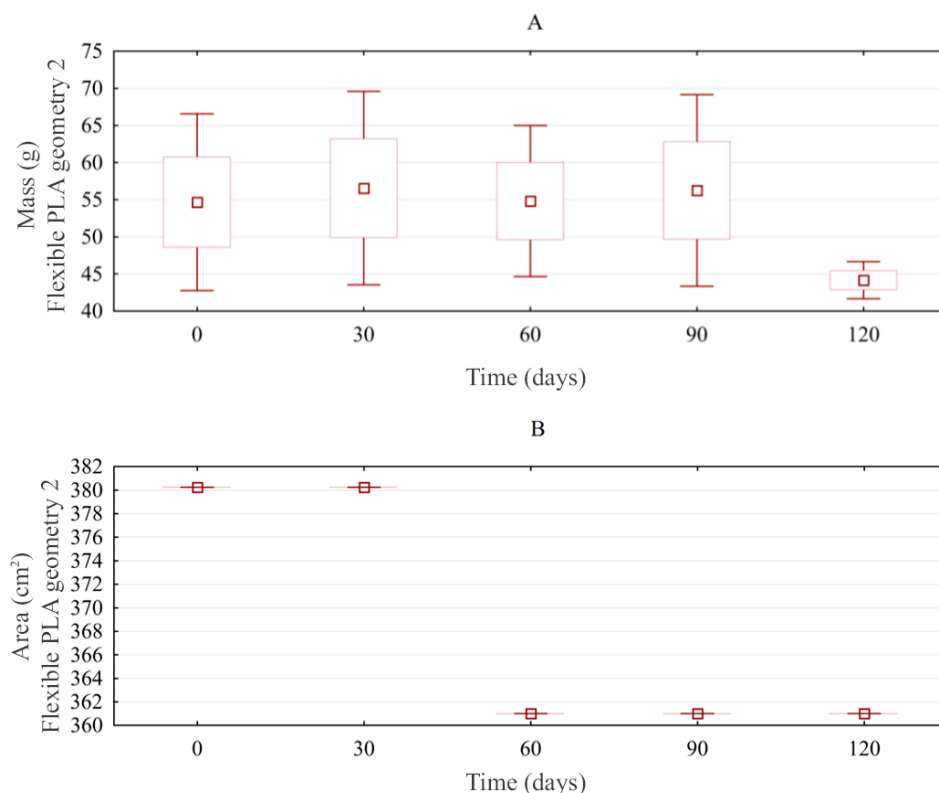
Figure 10 – Analysis of the (A) loss of mass (g) and (B) area (cm 2 ) by degradation of 3D-printed flexible PLA biopolymer (geometry 2) buried for 0, 30, 60, 90, and 120 days.
