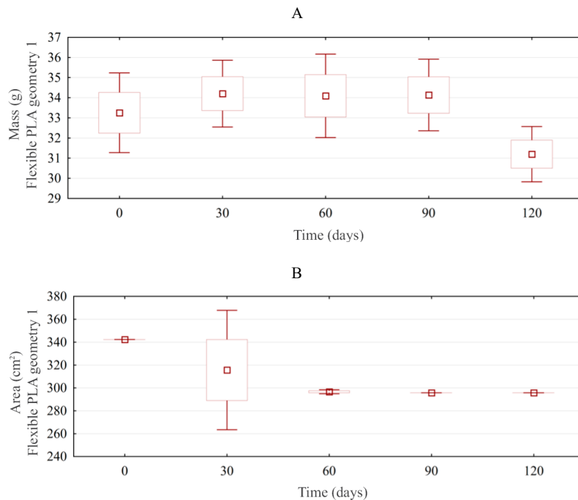
Figure 6 – Analysis of the (A) loss of mass (g) and (B) area (cm 2 ) by degradation of 3D-printed flexible PLA biopolymer (geometry 1) buried for 0, 30, 60, 90, and 120 days.
