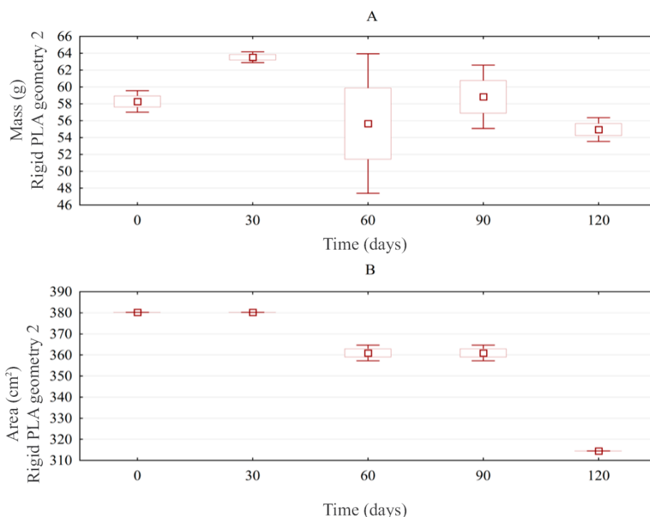
Figure 12 – Analysis of the (A) loss of mass (g) and (B) area (cm 2 ) by degradation of 3D-printed rigid PLA biopolymer (geometry 2) buried for 0, 30, 60, 90, and 120 days.
