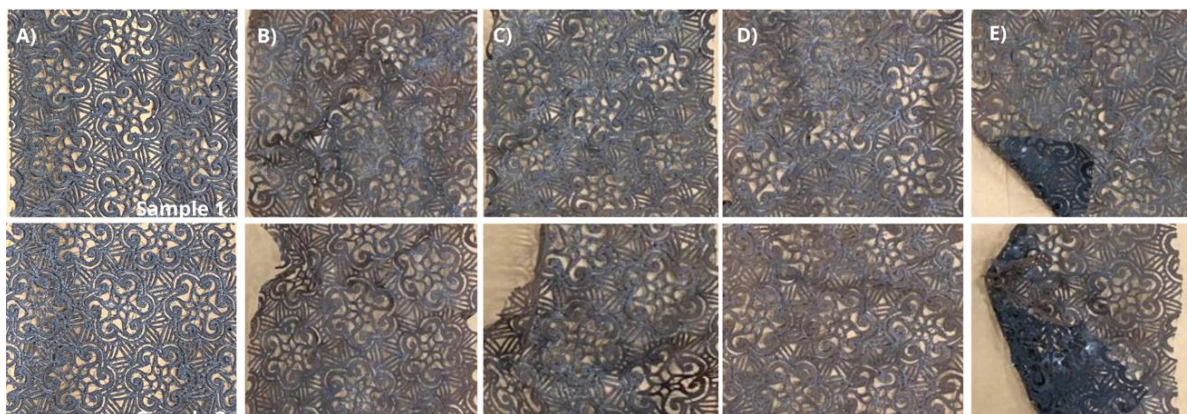
Figure 15 – Degradation process of 3D-printed flexible PLA biopolymer samples (geometry 3) buried for (A) 0, (B) 30, (C) 60, (D) 90, and (E) 120 days.
