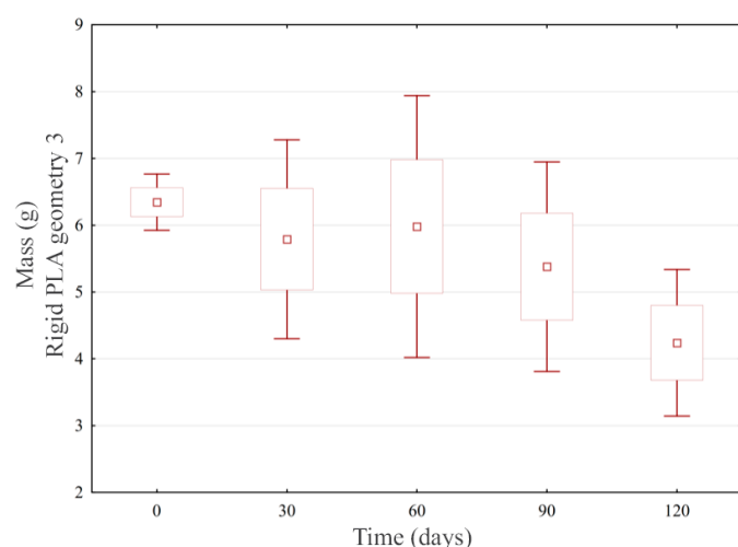
Figure 16 – Analysis of the (A) loss of mass (g) by degradation of 3D-printed rigid PLA biopolymer (geometry 3) buried for 0, 30, 60, 90, and 120 days.
