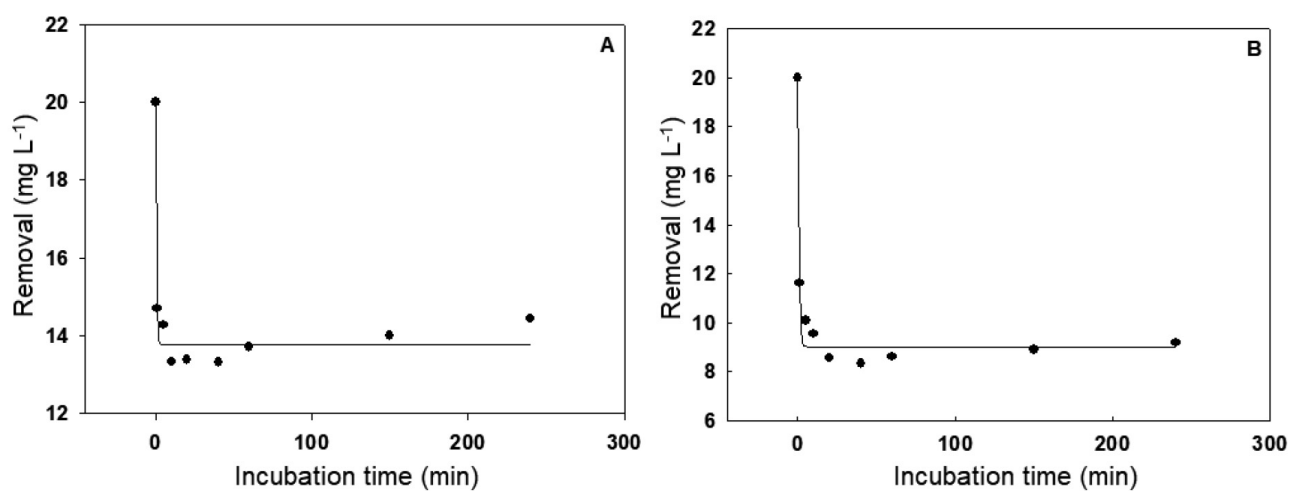
Figure 3 – Regression analysis for adsorption treatments with chitins obtained by methodologies (A) T7 and (B) T8.
