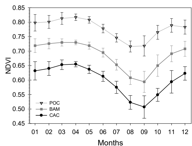
Figure 3 – Monthly average and standard deviation of the NDVI from the period 2000-2016, in three areas of study, Cáceres (CAC), Poconé (POC) and Barão de Melgaço (BAM), in the northern region of the Pantanal in the State of Mato Grosso.
