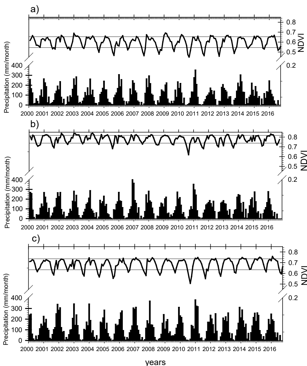
Figure 2 – Monthly seasonal change of NDVI and Precipitation of the period 2000-2016, the line (in black) represents the lower and higher limits of the standard deviation of the period average. (A) Cáceres – CAC, (B) Poconé – POC, and (C) Barão de Melgaço – BAM, in the northern region of the Pantanal in the State of Mato Grosso.
