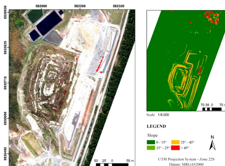
Figure 6 – Terrain declivity in the survey on 05/05/2018. Source: Cunha (2020).
