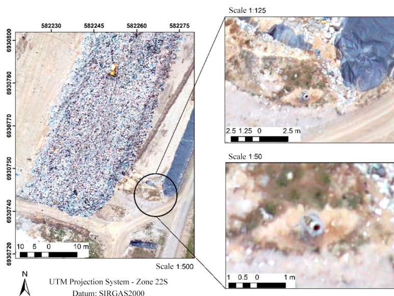
Figure 3 – Analysis of components at different scales of proximity. Source: Cunha (2020).
