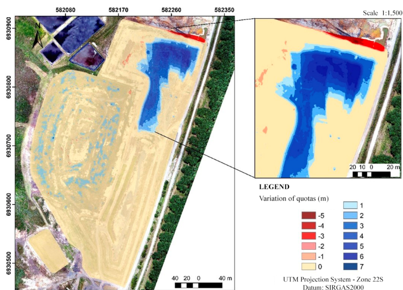
Figure 11 – Changes in the quotas of the massifs between the second and third surveys.
