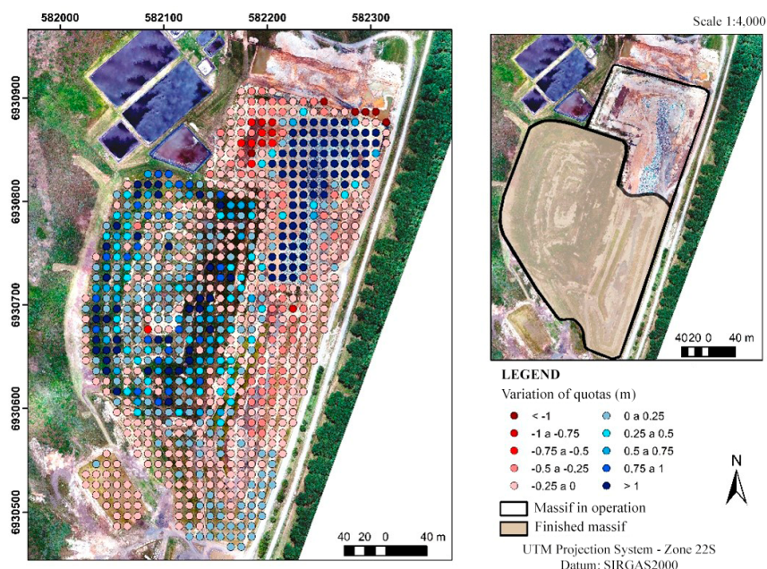
Figure 10 – Monitoring of settlement between the surveys on 09/05/2018 and 02/13/2018.
