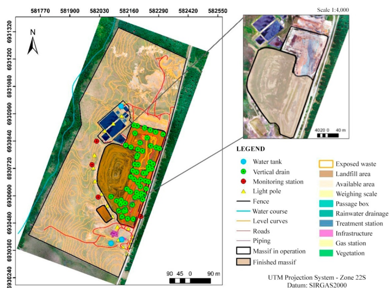
Figure 4 – Planialtimetric map of the survey on 02/13/2019. Source: Cunha (2020).
