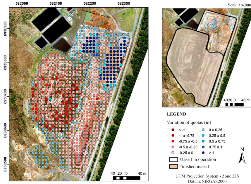
Figure 8 – Monitoring of settlement between the surveys on 05/05/2018 and 09/05/2018. Source: Cunha (2020).
