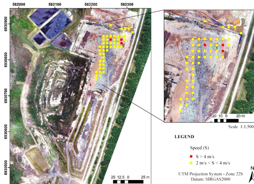
Figure 13 – Distribution of the settlement speeds between 09/05/2018 and 02/13/2019. Source: Cunha (2020).
