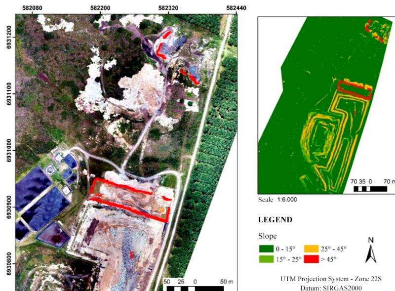
Figure 7 – Terrain declivity in the survey on 02/13/2019.
