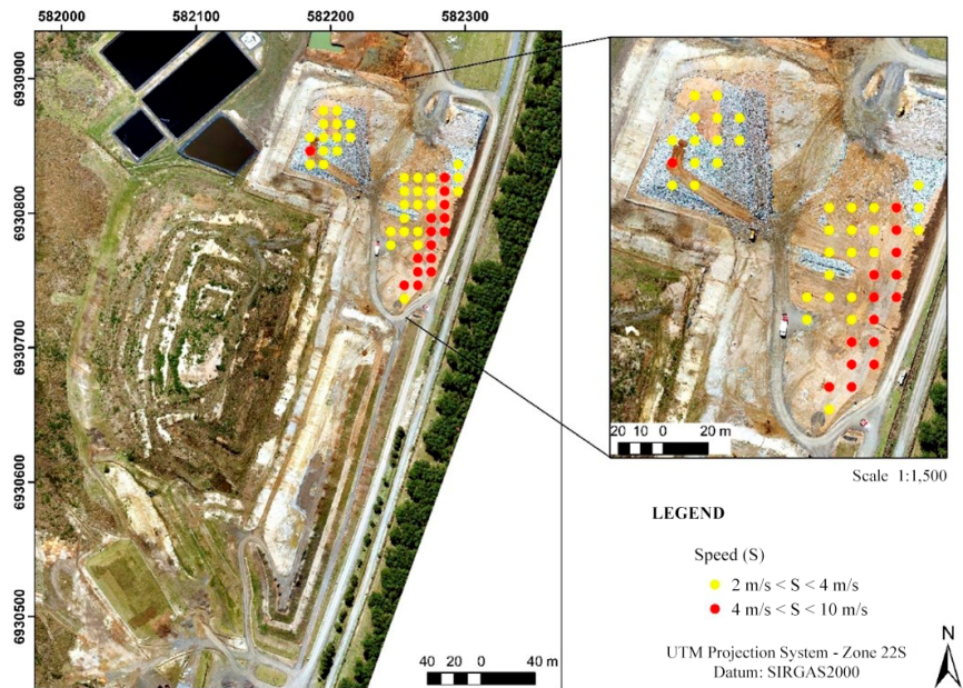
Figure 12 – Distribution of settlement speeds between 05/05/2018 and 09/05/2018. Source: Cunha (2020).
