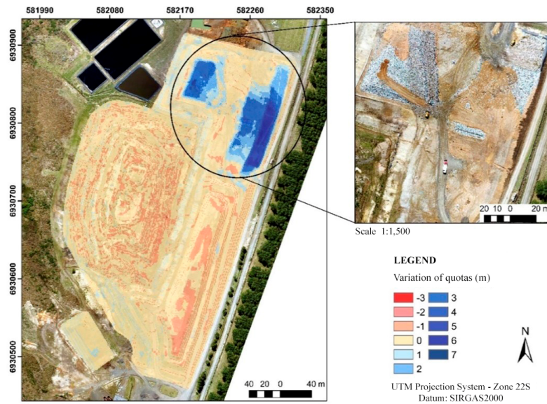
Figure 9 – Changes in the quotas of the massifs between 05/05/2018 and 09/05/2018. Source: Cunha (2020).
