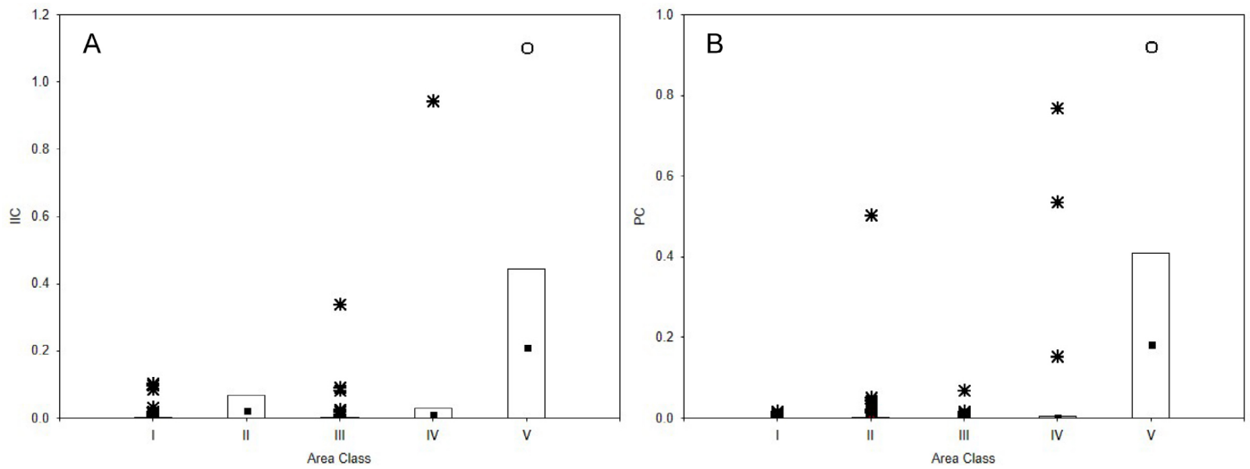
Figure 5 – Variation values of connectivity of the Tarumã-Açu basin fragments (based on 100 m dispersion threshold) by size class, according to: (A) Integral Connectivity Index; (B) Probability of Connectivity. The columns show the mean and the variation of the indexes, while the asterisks and circles indicate outliers and very discrepant values, respectively.
