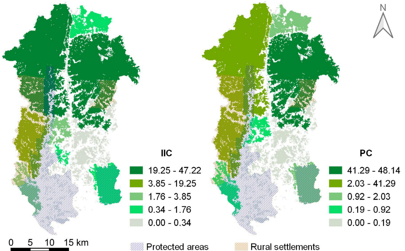
Figure 6 – Classification of remaining forest patches in the Tarumã-Açu River basin under 100 m dispersion threshold, based on the importance for connectivity determined by the Integral Connectivity Index (IIC) and the Probability of Connectivity (PC).
