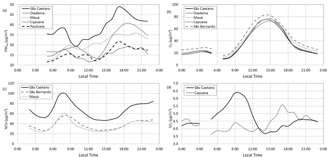
Figure 4 – Mean diurnal cycle for (A) PM_{10} , (B) O_3 , (C) NO_x and (D) SO_2 at five ABC stations in 2015. There is a lack of data at certain hours of the day because of automated instrumental checks in the monitoring stations. Note: SO_2 measurements at Capuava were available only between August and December.
