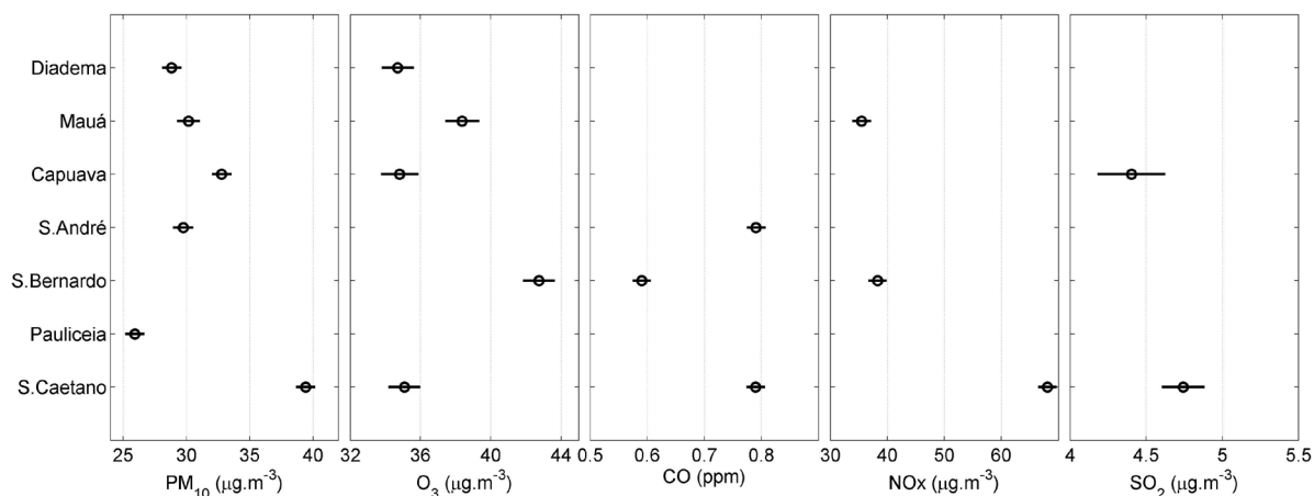
Figure 2 – Analysis of Variance (ANOVA) applied to daily mean concentrations of PM_{10} , O_3 , CO, NOx and SO_2 at seven air quality monitoring sites in the ABC region in 2015. Circles indicate the mean concentration values for each pollutant at each site. Error bars represent the overall confidence level for each pollutant, considering the variability at all sites. The difference in the mean concentration of a pollutant between pairs of stations is statistically significant ( p < 0.05 ) when the error bars do not overlap. Note: SO_2 measurements at Capuava were available only between August and December.
