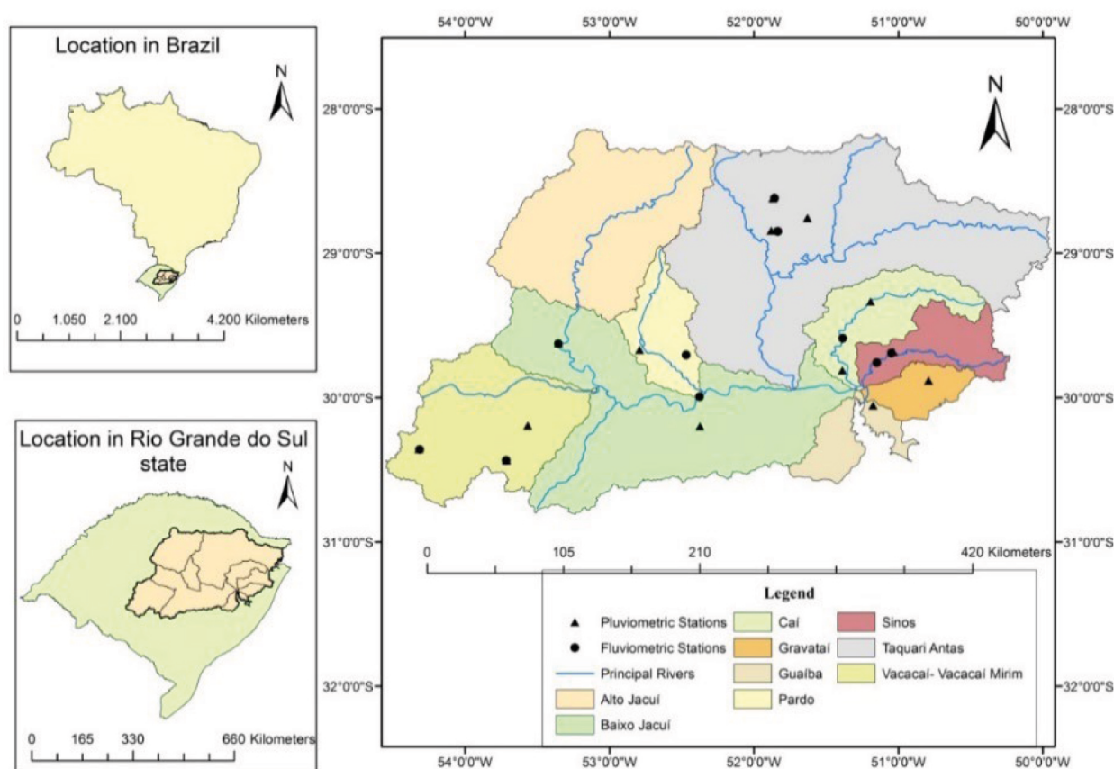
Figure 1 – Location of the Guaíba Hydrographic Region and spatialization of the hydrological stations.
