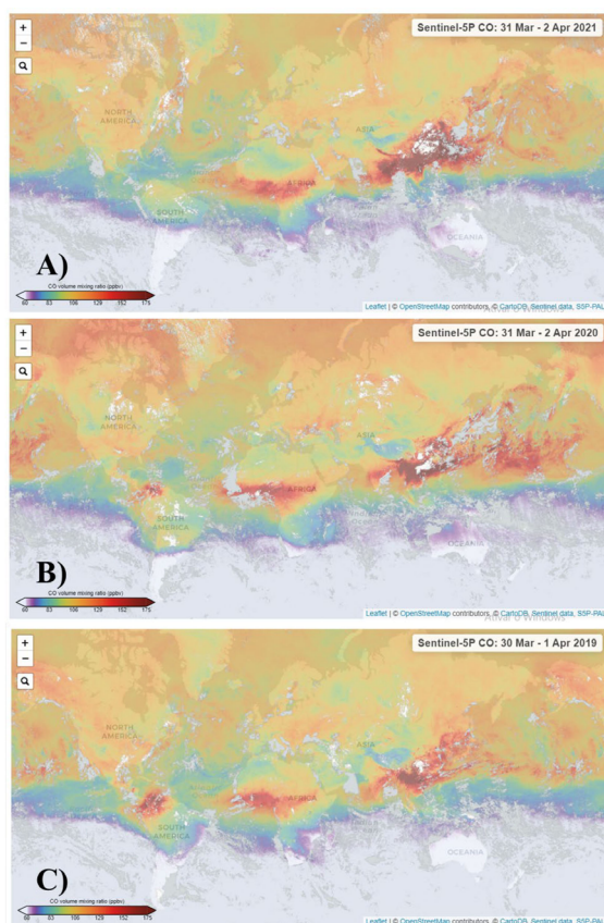
Figure 1 – Map of air quality (CO) around the world: (A) during the COVID-19 pandemic [March to April 2021], (B) during the COVID-19 pandemic [March to April 2020], and (C) before the pandemic [March to April 2019].
