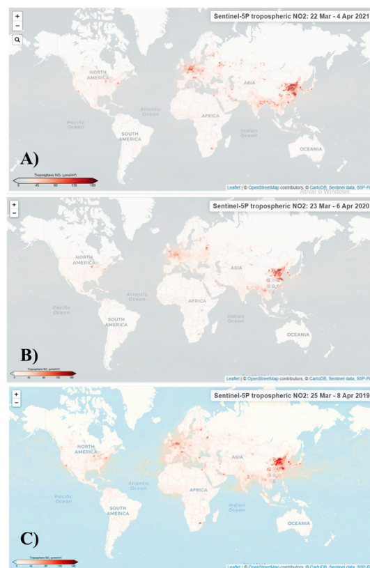
Figure 2 – Map of air quality ( \text{NO}_2 ) around the world: (A) during the COVID-19 pandemic [March to April 2021], (B) during the COVID-19 pandemic [March to April 2020], and (C) before the pandemic [March to April 2019].
