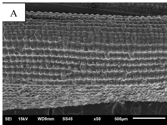
Figure 2 – SEM analysis; (A) RH and (B) RHA.
