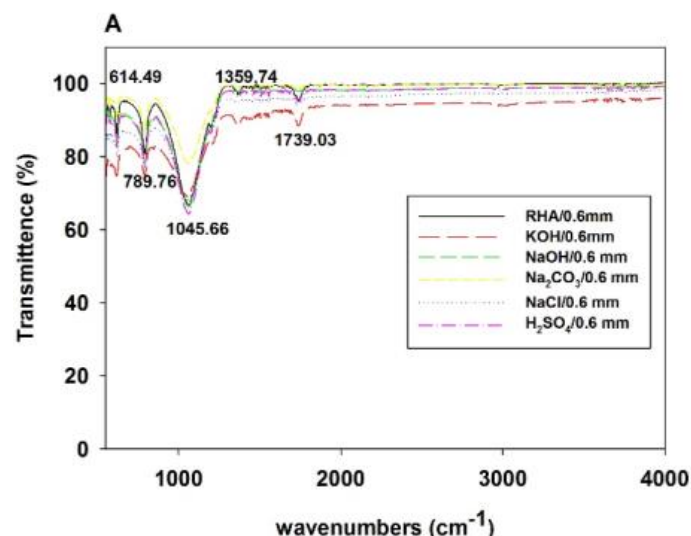
Figure 3 – Infrared spectra of the raw and treated ash; (A) grain size 0.6 mm and (B) grain size 1 mm.
